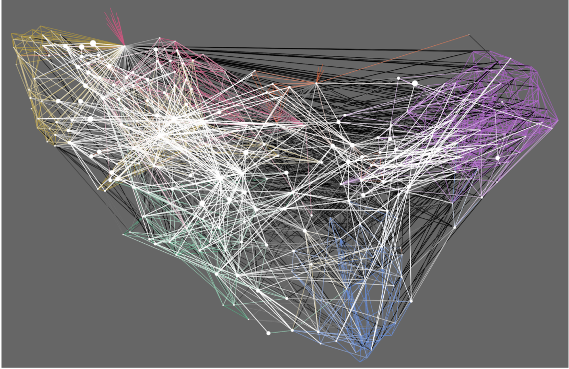
Figure 3: Visualization of the ambiguity of modularity clustering on the C. Elegans network, consisting of a nematode's neurons and their connections [21]. Layout Force Atlas 2.
