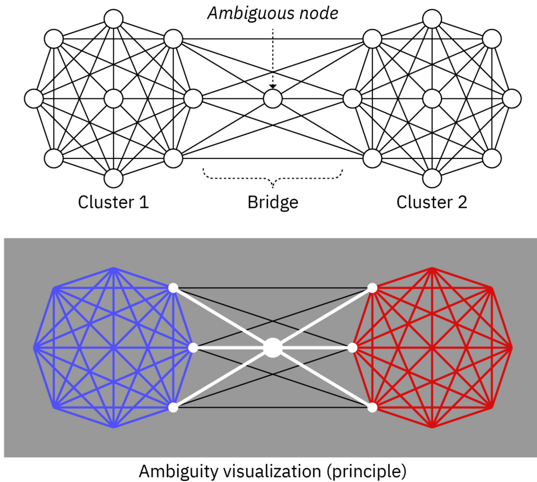
Figure 1: Principle of the visualization. Black edges are consistently bridging over different clusters. Colored nodes and edges are consistently within the same cluster. White nodes and edges are sometimes bridging, sometimes within the same cluster, depending on random factors in the community detection algorithm.
