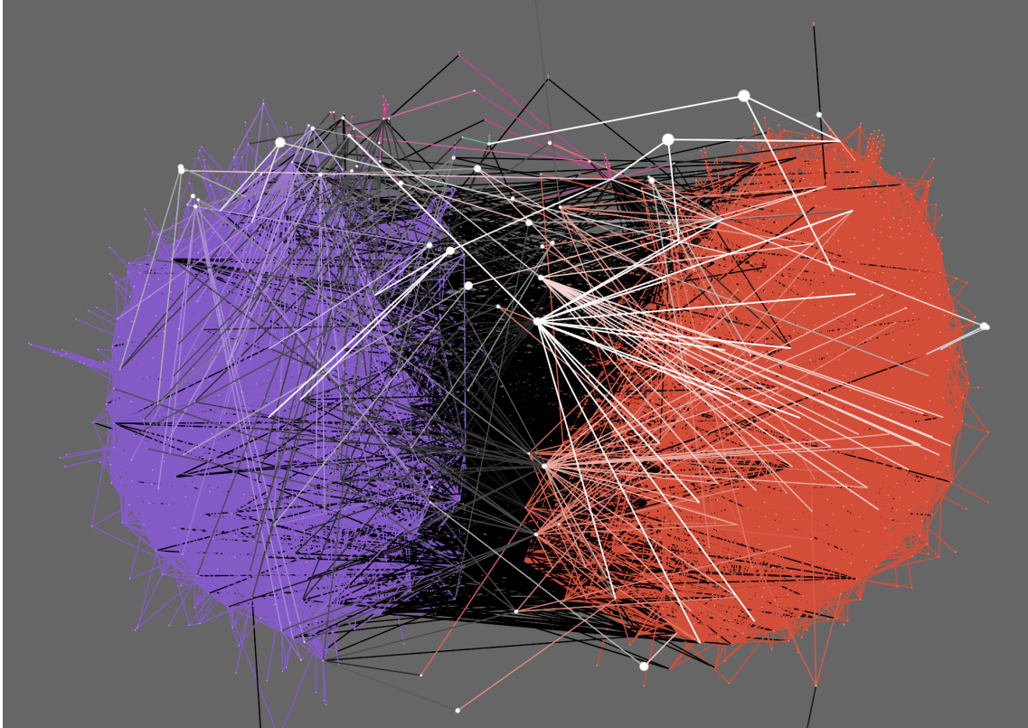
Figure 2: Visualization of the ambiguity of modularity clustering on the network from Divided they Blog [1], representing the US political blogosphere in 2024, structured in two clusters. Layout Force Atlas 2 [10].
