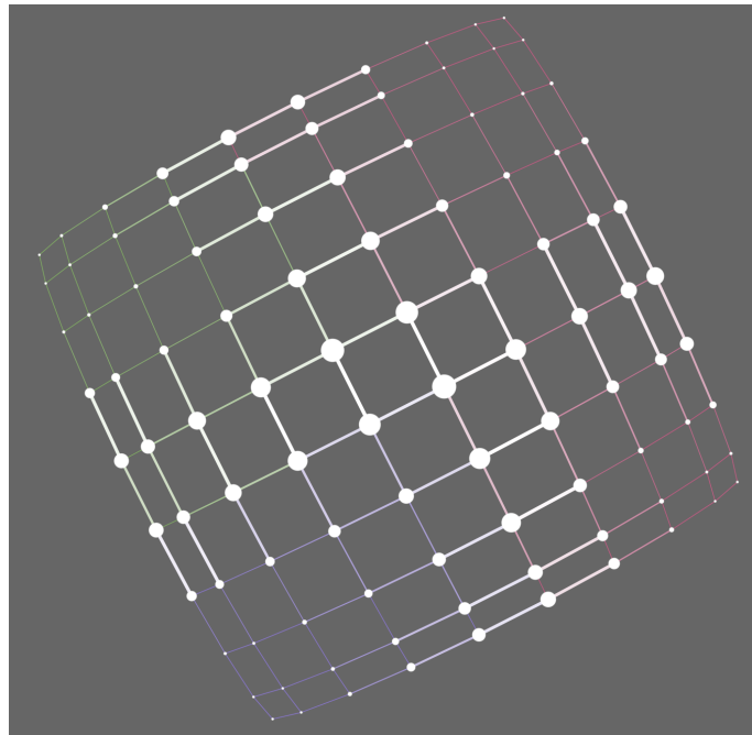
Figure 4: Visualization of the ambiguity of modularity clustering on a square lattice (a simple mathematical grid). Layout Force Atlas 2.
